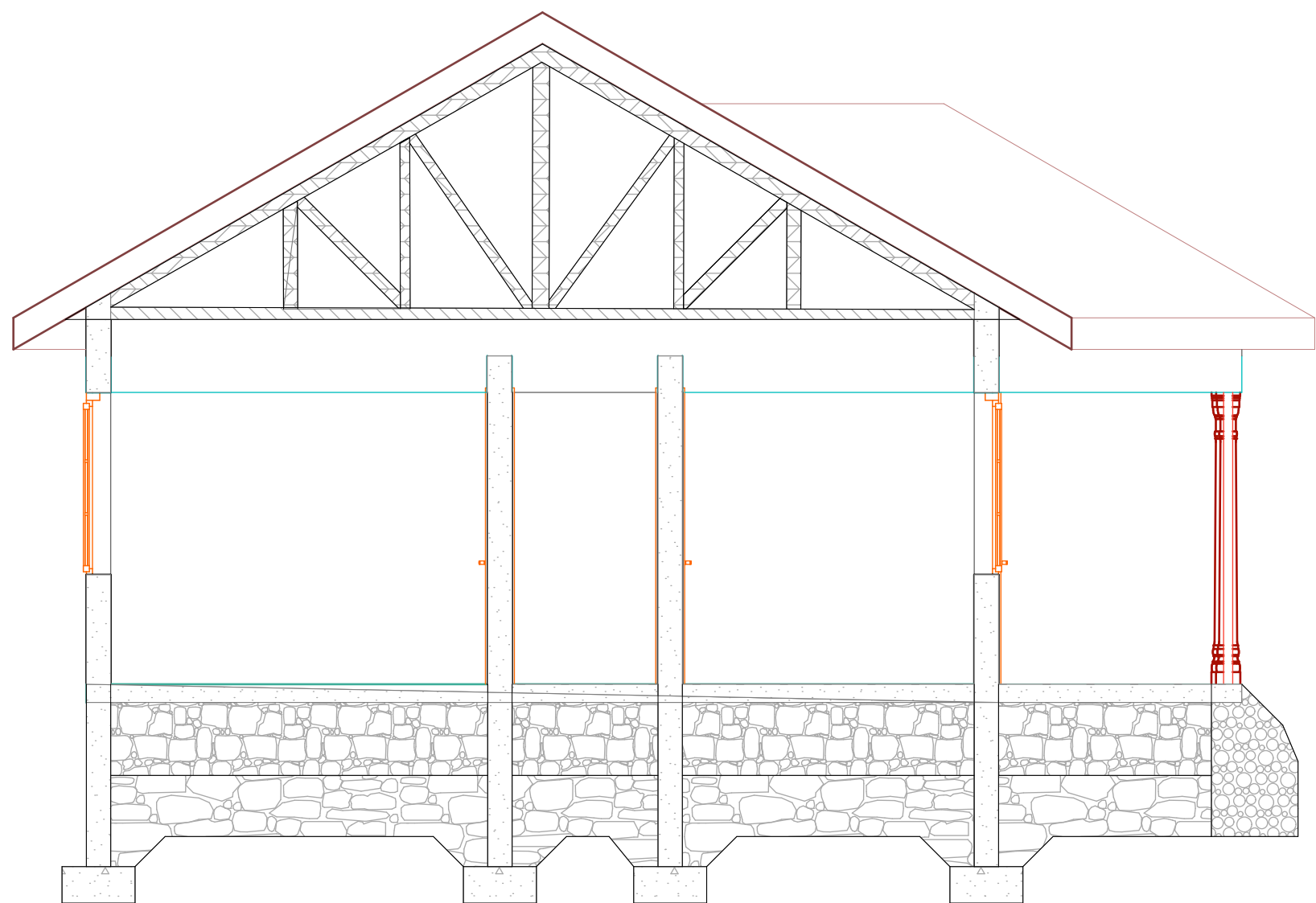
SECTION S-01
