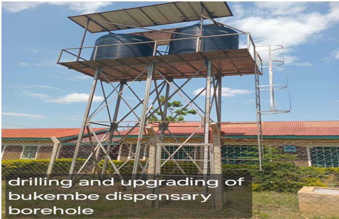
Drilled and upgraded borehole into solar pumping system at Bukembe Dispensary
